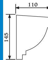
Product P115 Uni-Shape Parapet Profile Length: 3m
