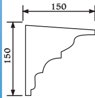
Product PP2 Uni-Shape Parapet Profile N° 2082 Length: 3m
