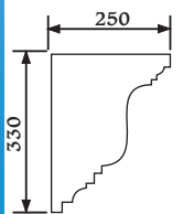
Product S113 Uni-Shape Stringer Profile Length: 3m
