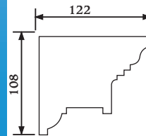
Product PP9 Uni-Shape Parapet Profile N° 3083 Length: 3m
