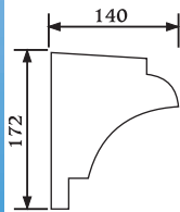
Product S110 Uni-Shape Stringer Profile Length: 3m
