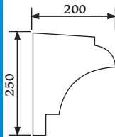
Product P105 Uni-Shape Parapet Profile Length: 3m
