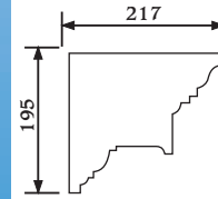
Product PP8 Uni-Shape Parapet Profile N° 3082 Length: 3m
