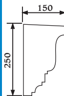
Product P106 Uni-Shape Parapet Profile Length: 3m
