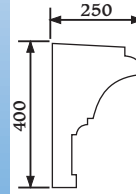
Product P108 Uni-Shape Parapet Profile Length: 3m
