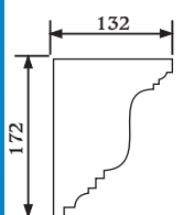
Product S116 Uni-Shape Stringer Profile Length: 3m
