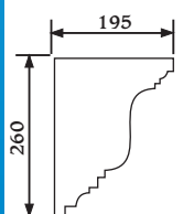
Product S115 Uni-Shape Stringer Profile Length: 3m
