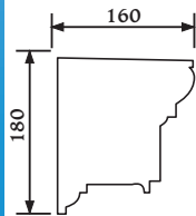
Product PP3 Uni-Shape Parapet Profile N° 2083 Length: 3m
