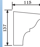
Product PP7 Uni-Shape Parapet Profile N° 3081 Length: 3m
