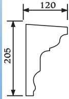
Product PP1 Uni-Shape Parapet Profile N° 2081 Length: 3m
