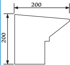
Product PP4 Uni-Shape Parapet Profile N° 2084 Length: 3m
