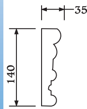
Product AM110 Uni-Shape Architraves Profile Length: 3m
