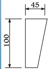
Product AM103 Uni-Shape Architraves Profile Length: 3m
