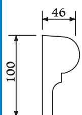
Product AM109 Uni-Shape Architraves Profile Length: 3m
