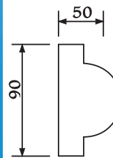
Product AM106 Uni-Shape Architraves Profile Length: 3m
