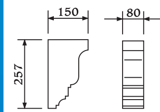
Product BRK 101 Console Bracket Profile
