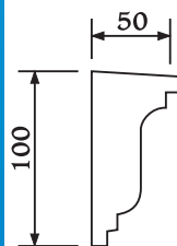
Product AM107 Uni-Shape Architraves Profile Length: 3m
