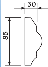
Product AM102 Uni-Shape Architraves Profile Length: 3m
