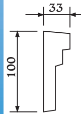
Product AM111 Uni-Shape Architraves Profile Length: 3m
