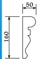
Product AM112 Uni-Shape Architraves Profile Length: 3m
