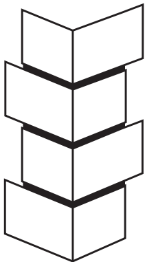
Stepped Quoin Large panel: 380 x 260 mm Small panel: 260 x 260 mm Height: 2600mm (8 panels high)
