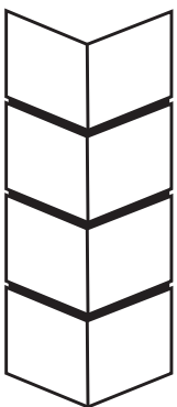
V-Joint Quoin Sizes: 300 X 300 x 2700mm 350 X 300 x 2700mm 450 X 300 x 2700mm (All 9 panels high)
