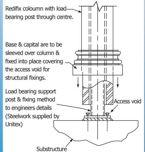
COLUMN INSTALLATION DETAILS (Top of column similar)
