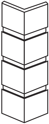
Square-Joint Quoin 300 X 300 x 2700mm (9 panels high)
